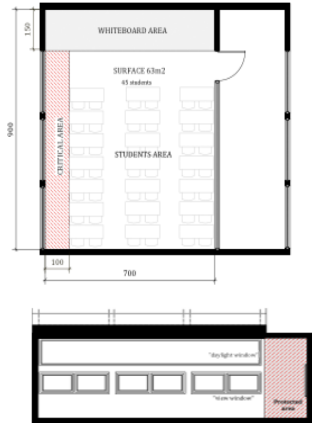
Fig. 3 Classroom plans that portray the increase on the classroom surface, with and without critical area.
