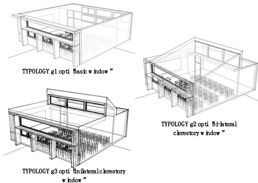
Fig. 4 3D models of east and west-facing typologies.
