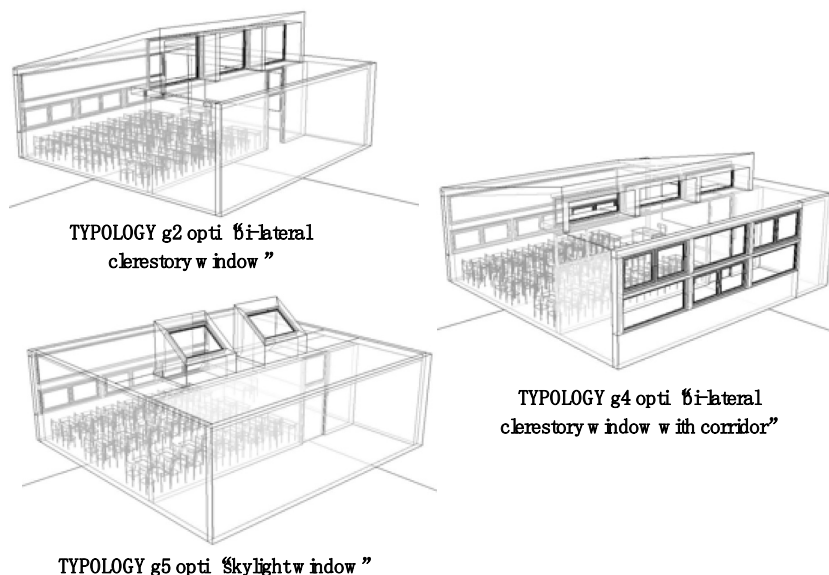
Fig. 3 3D models of south-facing typologies.
