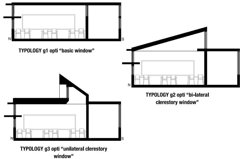
Fig. 2 Sectional cut of north-facing typologies.
