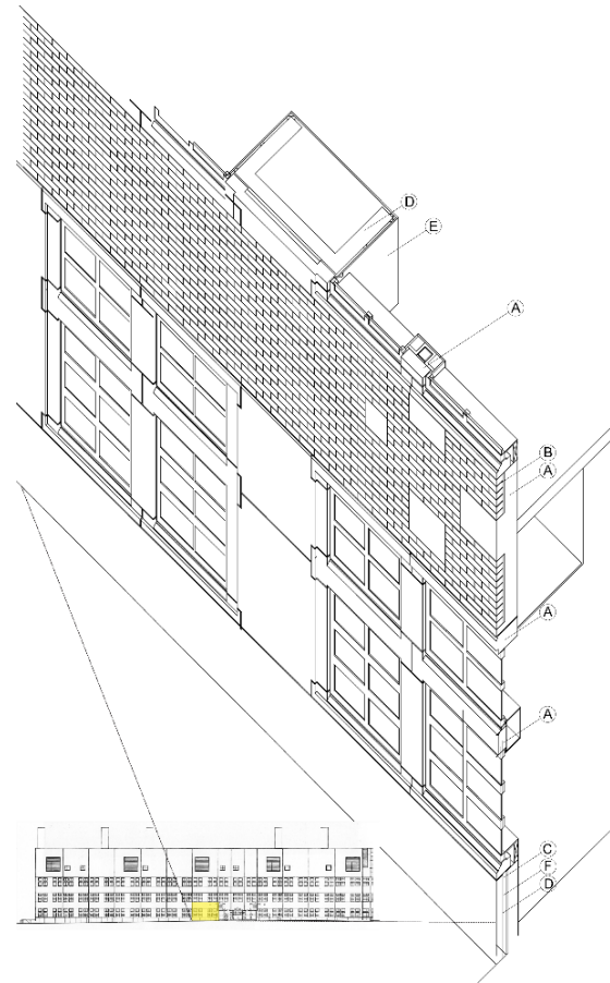
Fig. 2 Diagram of the claddings of the partly wall section of the LTL.
