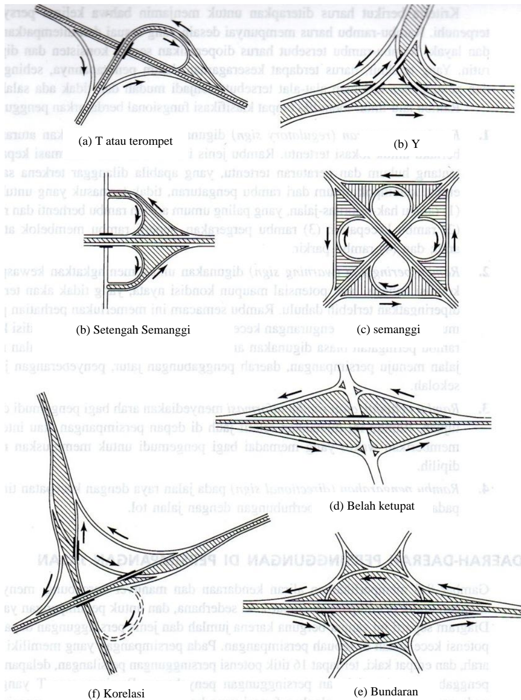
Figure 2.1 Types of interchange.
