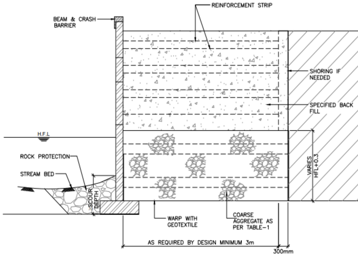
Figure 1. Typical RE Wall in submerged condition.
