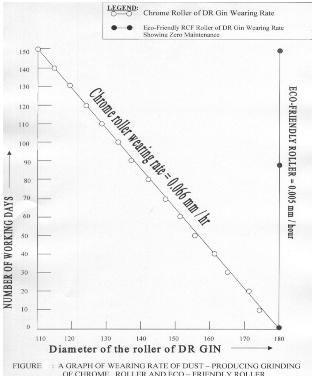
Figure 8. A graph of wearing rate of dust-producing grinding of CCLC roller and RCF roller.
