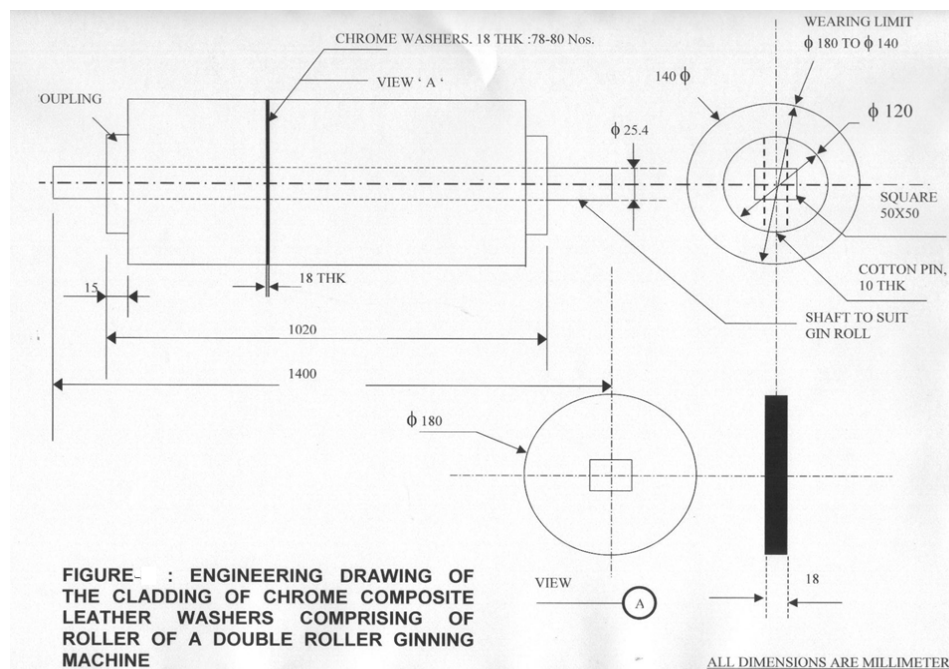
Figure 4. An engineering drawing of the cladding of chrome composite leather clad
