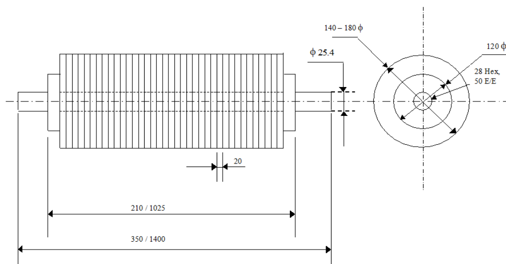
Figure 6. The assembly drawing of rubberized cotton fabric (RCF) washers for making RCF rollers of cotton double roller gins.
