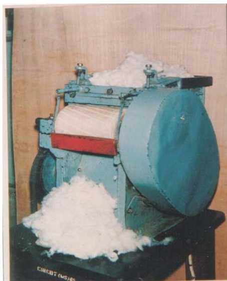
GRED ASSEMBLED WITH RCF LABORATORY ROLLER SUCCESSFULLY GINNING OUT SEED-COTTON
