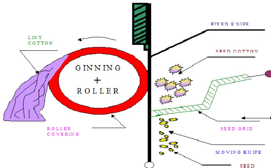
Figure 1. McCarthy principle of cotton roller ginning process.
