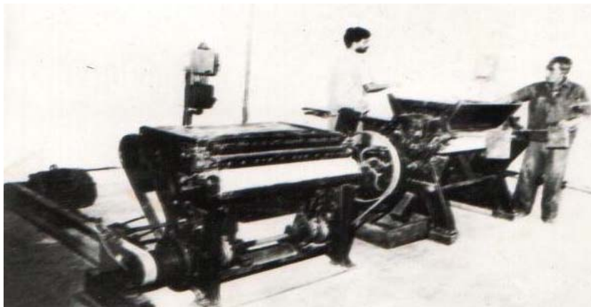
Figure 10. Single roller (SR) gin and double roller (DR) gin. Source: Central Institute for Research on Cotton Technology (Indian Council of Agricultural Research, Matunga, Mumbai, India).
