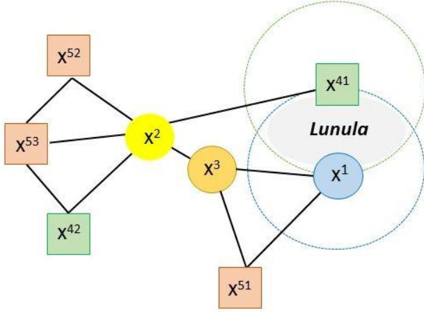
Fig. 1 RNG structure - Euclidean proximity measure - Associated adjacency matrix.
