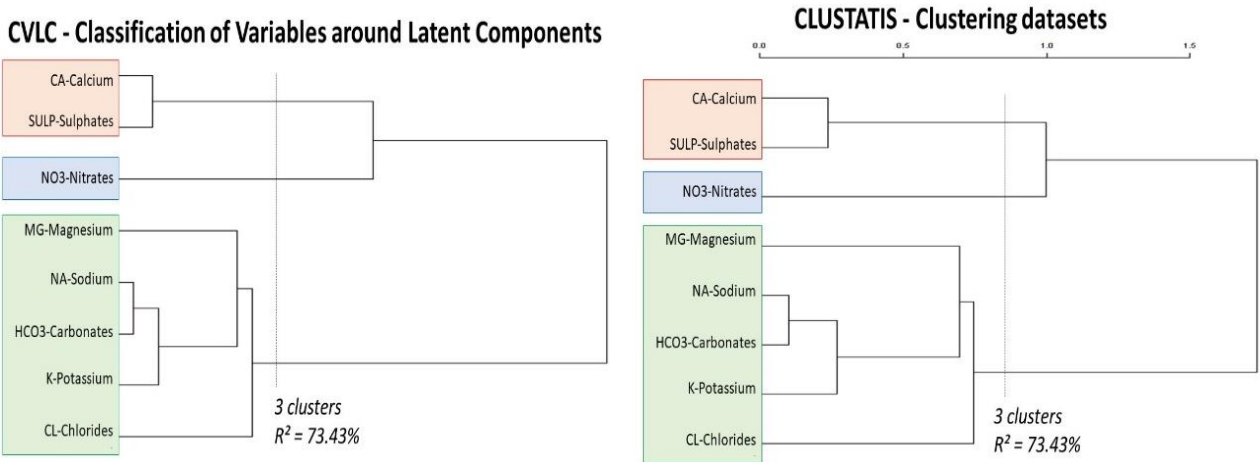
Fig. 5 CVLC and Clustatis dendrograms.
