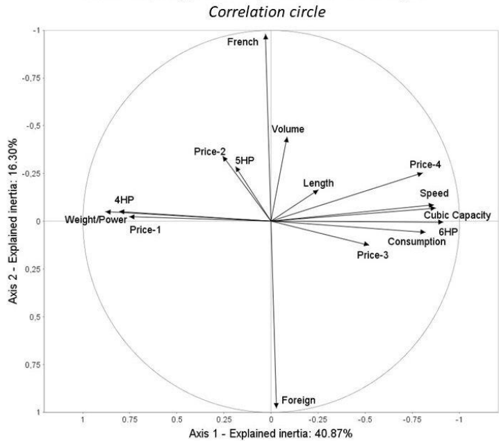
TPCA - Topological Principal Component Analysis
