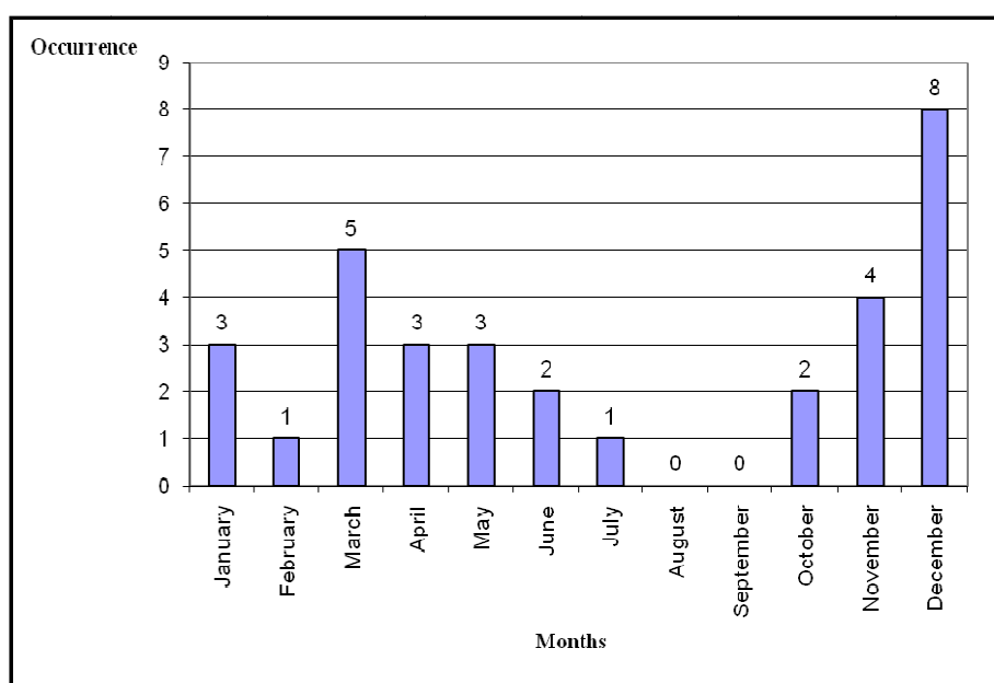
Fig. 9 The occurrence of floods per month between 1970 and 2015 (based on the 2010, 2016 archives of the Transcarpathian Hydrometeorological Centre [13, 14]).
