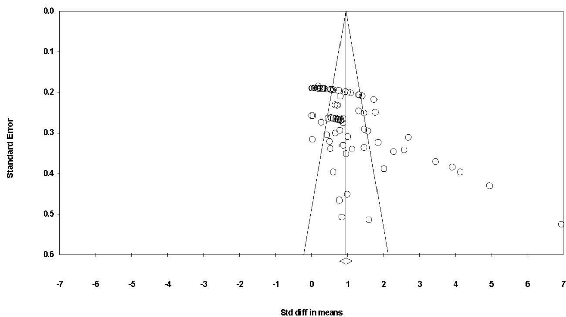
Figure 1. Funnel plot of standard error by standard differences in means under the random effects model.
