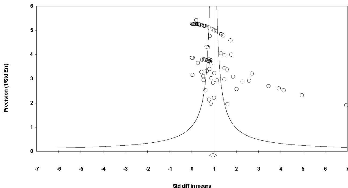
Figure 3. Funnel plot of precision by standard differences in means with imputed studies.
