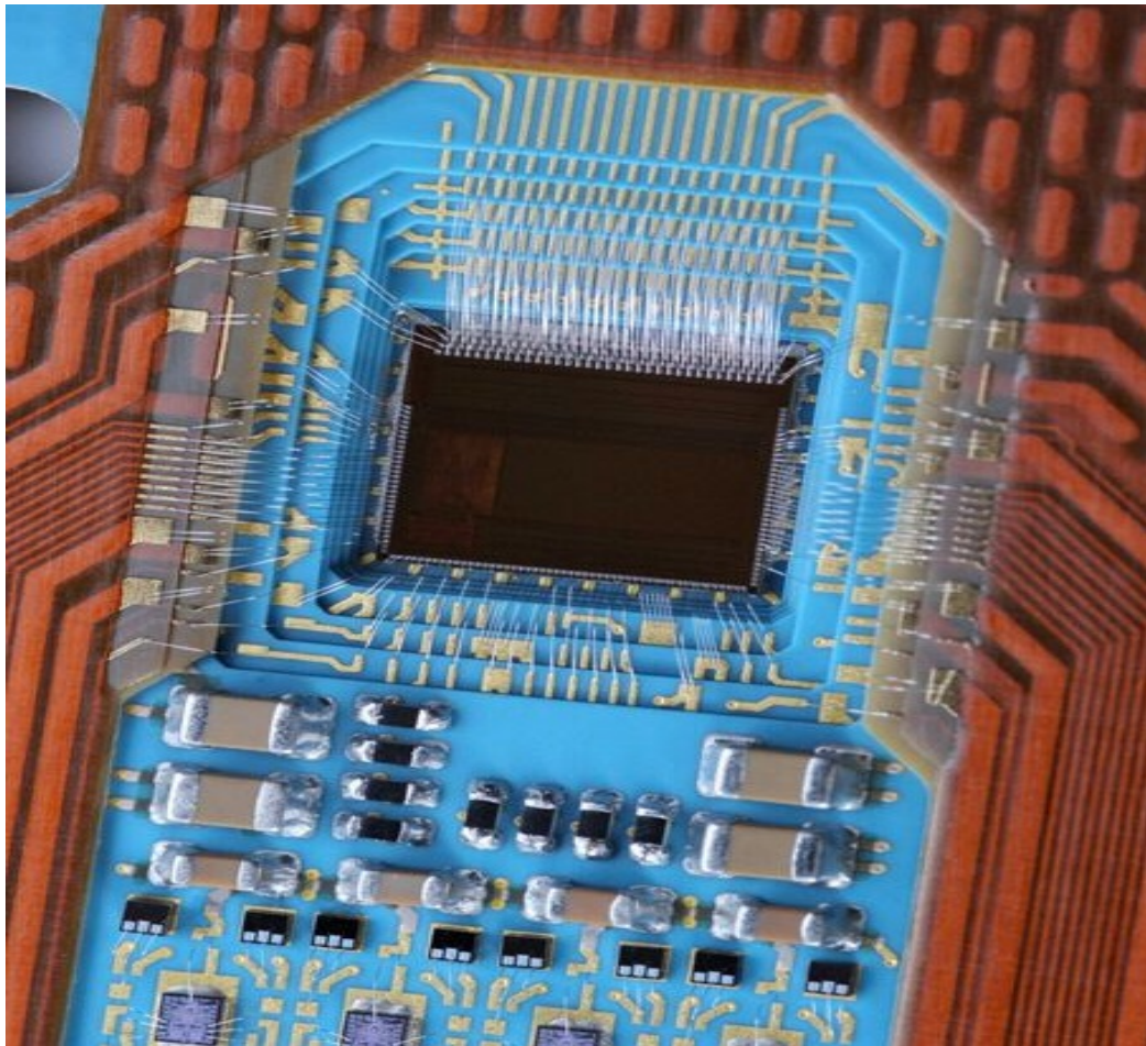
Fig. 6 Application 2—sensor chip—placed in LTCC cavity.
