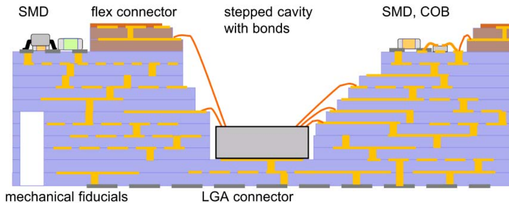
Fig. 7 Application 2—cross section.
