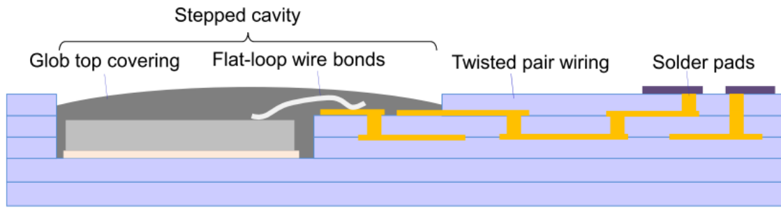
Fig. 3 Cross section and principle.
