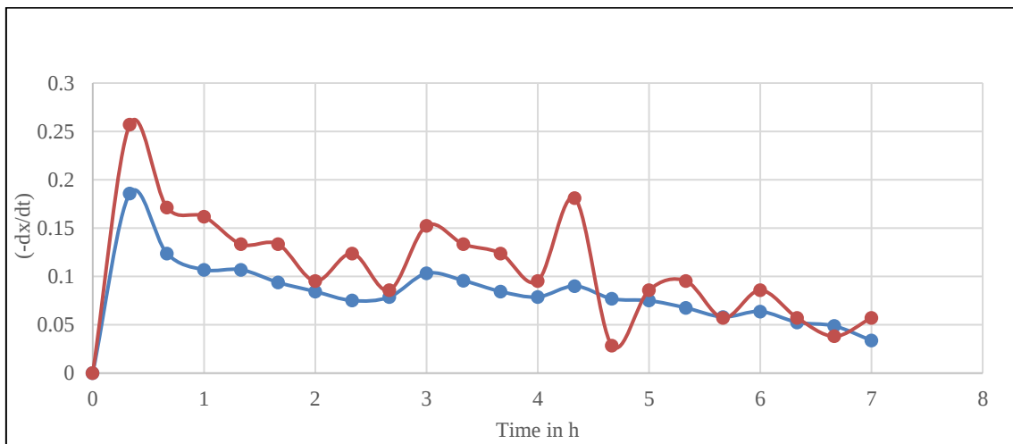
Fig. 16 Comparison of the drying rates of the big (the blue curve) and the small samples (the red curve).
