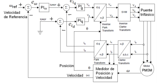
Fig. 3 Field oriented control (FOC) block diagram.
