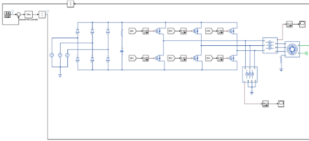
Fig. 4 Power control and controller part for a dc brushless motor.
