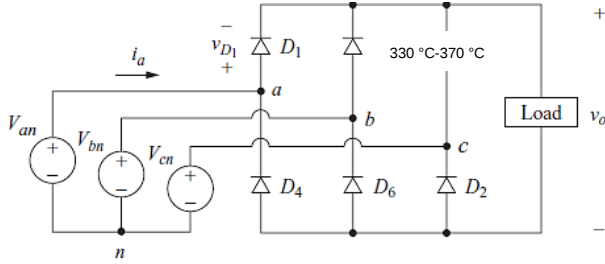
Fig. 1 Three phase full wave rectifier.
