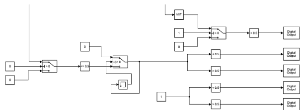
Fig. 10 Digital input and output signals.
