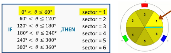
Fig. 6 Unmodulated rotor angular position sectors.
