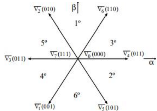
Fig. 2 Possible combinations of switched vectors.
