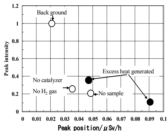
Fig. 7 The radiation emission peak position and intensity under various conditions.
