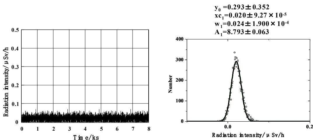
Fig. 3 (Left) Background change for \gamma -ray emissions. (Right) Intensity spectrum for the left graph.
