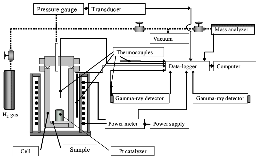
Fig. 1 Schematic drawing for the experimental set up.
