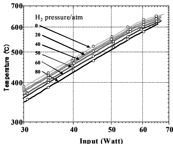
Fig. 2 Temperature dependence on heater power at different \text{H}_2 gas pressures.
