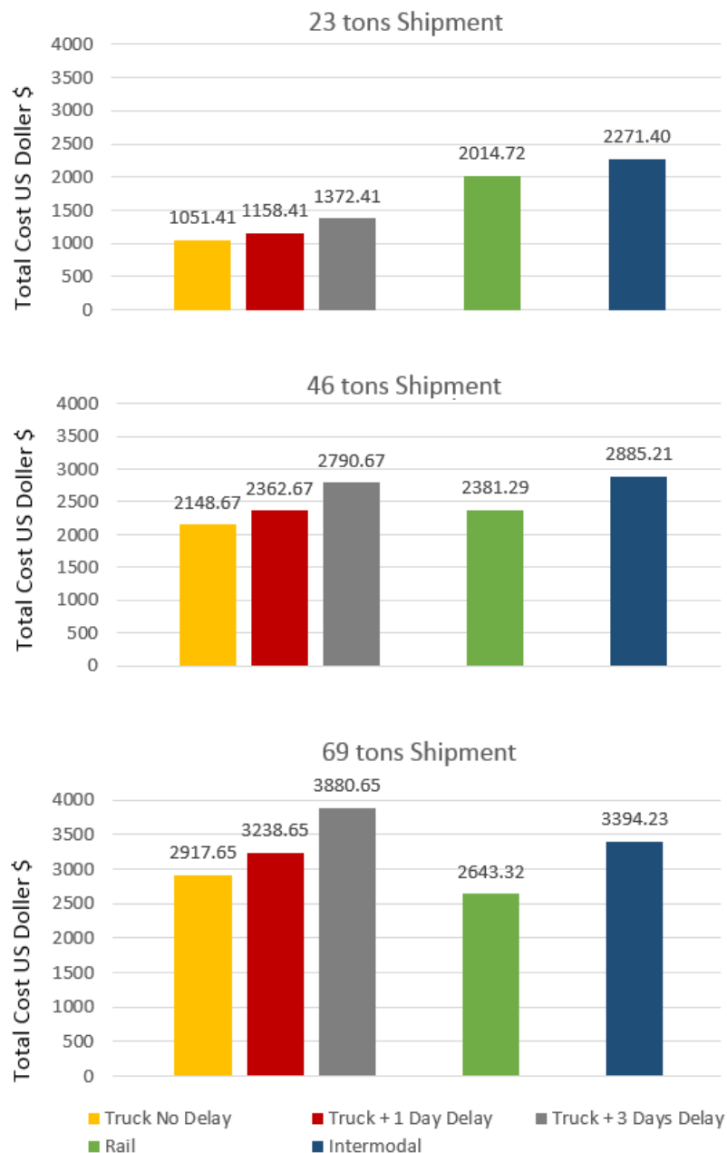
Fig. 7 Total Shipping cost of various shipment weight from Riyadh to Dubai using trucking, railway and intermodal systems.
