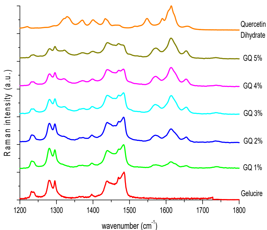
Fig. 8 Raman spectra of mixture Gelucire-quercetin (from 1% to 5%) in the spectral region 1,800-1,200 \text{cm}^{-1} at room temperature.
