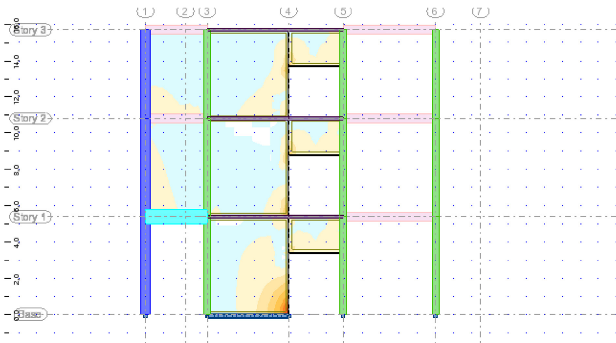
Fig. 9 Stresses in vertical direction for time 5.8 s. Acceleration in x direction.
