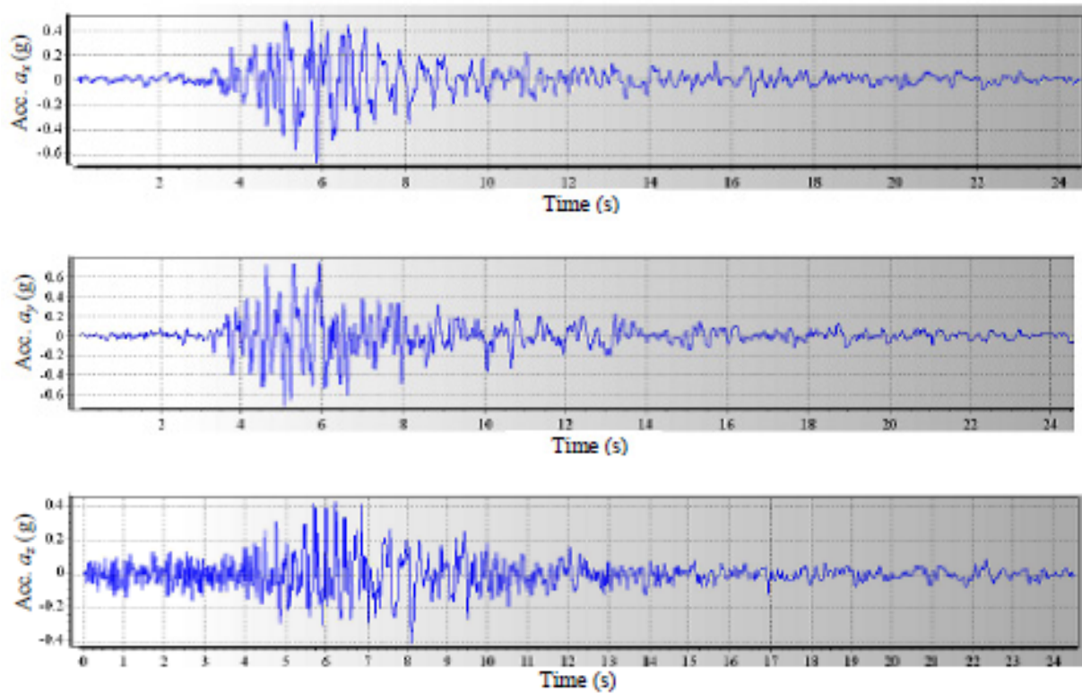
Fig. 8 Time history of acceleration in x, y and z direction for the Montenegro earthquake.
