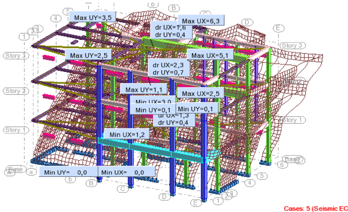
Fig. 5 Deformation of structure for earthquake motion in “x” direction.
