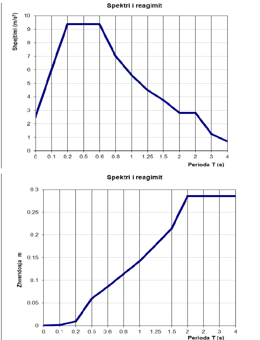
Fig. 4 Graphical view of the elastic acceleration and displacement spectrum for soil type C.
