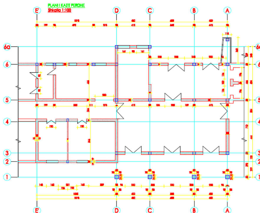
Fig. 2 Plan of the structure.
