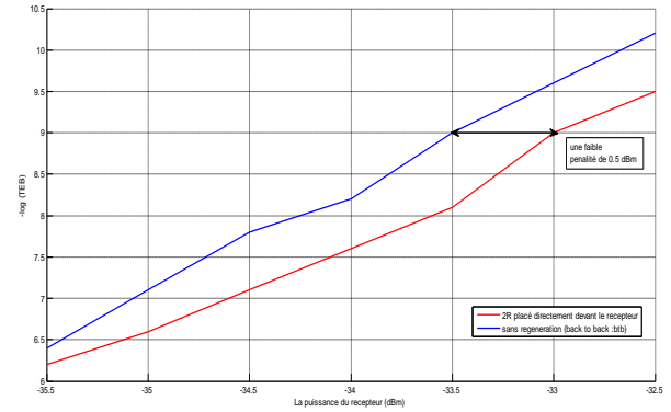
Fig 15 Evolution of the BER depending on the receiver power.
