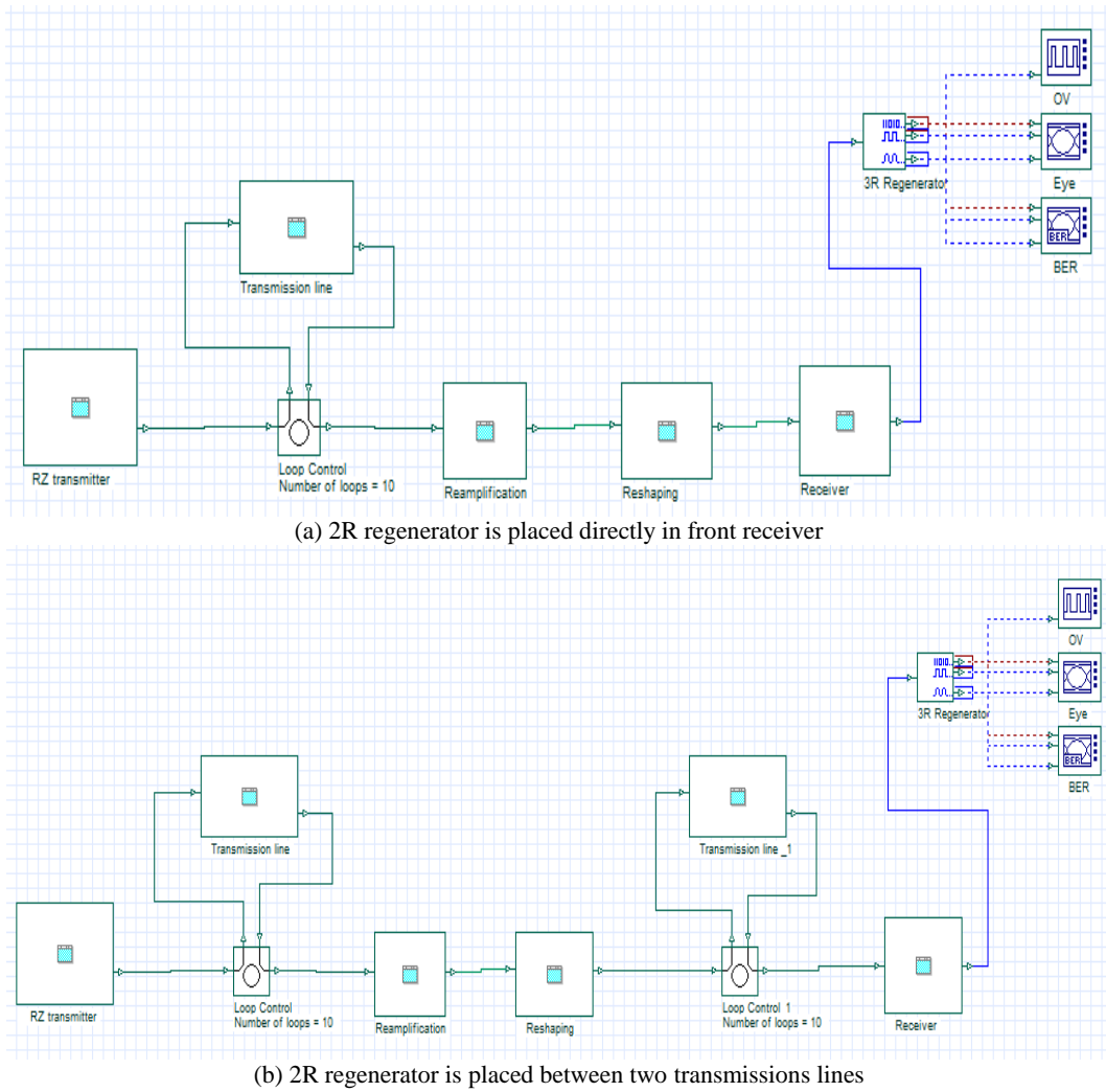
Fig. 3 Simulation setup of the proposed system.
