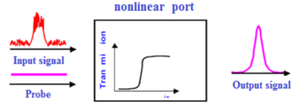
Fig. 2 Cross-2R regeneration.
