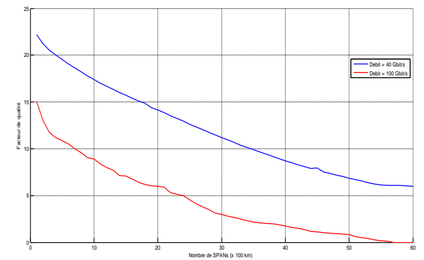
Fig 18 Quality factor based on the SPANs number (regenerator number).
