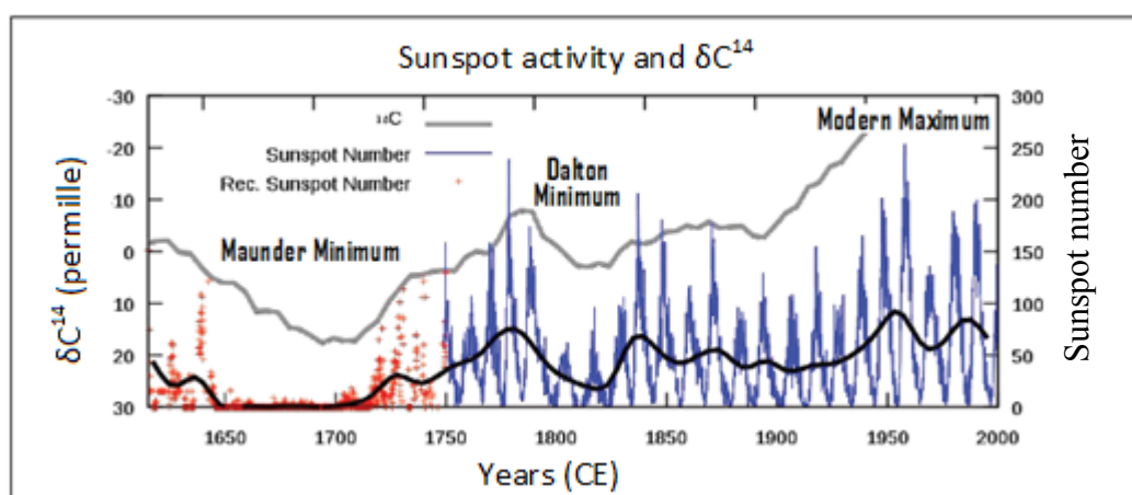
Fig. 2 The averages of annual group and Wolf sunspot number from 1600 until 2000, and \delta C^{14} , where the sunspot activity in y-axis in the right, \delta C^{14} in y-axis in left of the figure (from NOAA's Space Environment Center, http://www.swpc.noaa.gov ).
