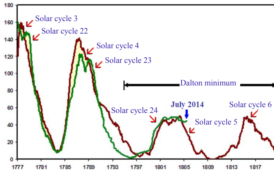
Fig. 5 Dalton Minimum Era and the solar cycles 22-24 are overlaid on solar cycles 3-5 above to show similarity, the date given until July 2014.
